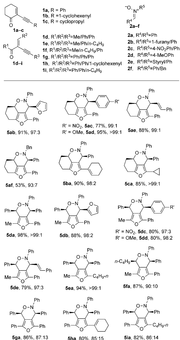
Figure 1. Gold(I)-catalyzed 1,3-dipolar [3+3] cycloaddition of 2-(1-alkynyl)-2-alken-1-ones 1 with nitrones 2 . The respective yields and diastereomeric ratios are given. Reaction conditions: 1 (0.4 mmol), nitrone 2 (0.44 mmol, 1.1 equiv), catalyst (2.5 mol %), CH 2 Cl 2 (4 mL), RT, 10–30 min.
