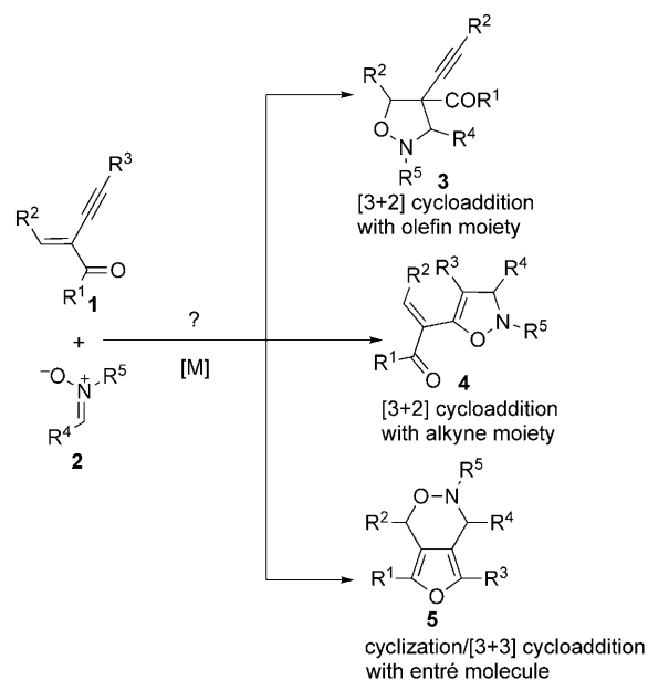
Scheme 1. Proposed metal-catalyzed cycloaddition of 2-(1-alkynyl)-2-alken-1-ones 1 with nitrones 2 .
