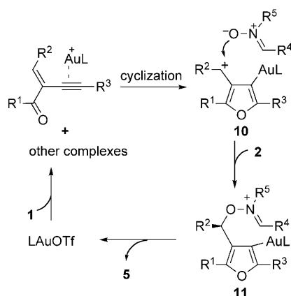
Scheme 5. Plausible mechanism for this gold(I)-catalyzed transformation.
