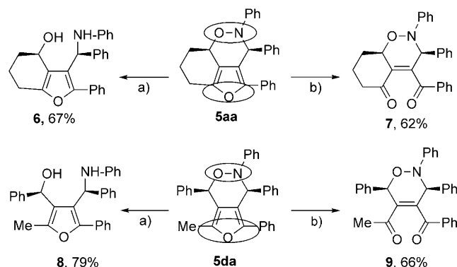
Scheme 4. Chemoselective ring-opening of furo[3,4- d ][1,2]oxazines provides efficient access to highly functionalized furans or 1,2-oxazines. Reaction conditions: a) \text{SmI}_2 , THF, 40°C; b) CAN, \text{CH}_3\text{CN}/\text{H}_2\text{O} 1:1, RT.
