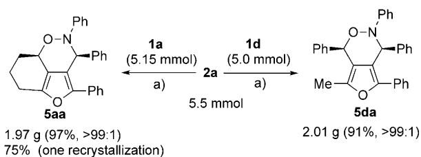
Scheme 2. Cyclization of 1a and 1d with 2a on a 5 mmol scale using only 0.2 mol % of the catalyst. Reaction conditions: a) Ph 3 PAuOTf (0.20 mol %), CH 2 Cl 2 , RT, 20 min.
