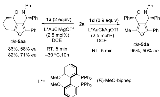
Scheme 3. Asymmetric gold-catalyzed [3+3] cycloaddition. DCE = 1,2-dichloroethane, Tf = trifluoromethanesulfonyl.
